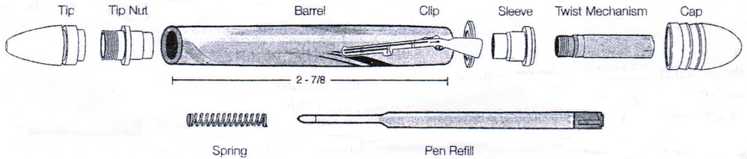
DIAGRAM C / Pen assembly
